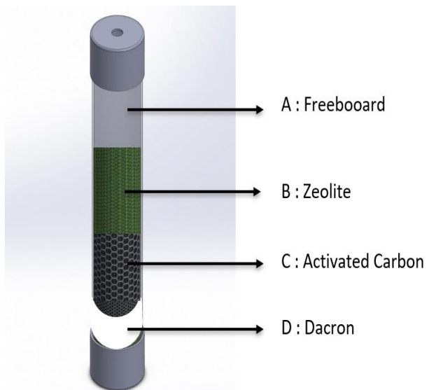
Figure 2. Filter Materials in Detail (this study)
