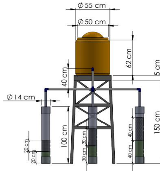
Figure 1. Filter Reactor
