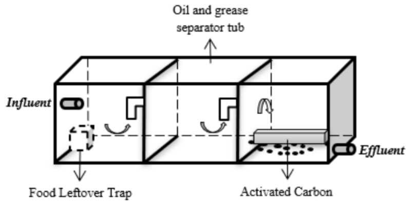
FIGURE 1. Modified grease trap (Zaharah et al, 2017)
