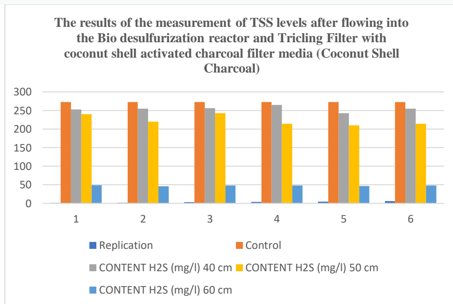
Graph 2 Reduction of TSS After flowing into the waste treatment plant, bio desulfurization and trickling filter
