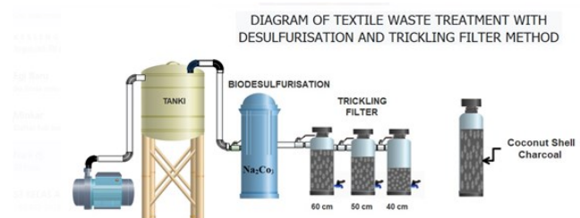
Picture of Bio Desulfurization Reactor and Trickling Filter
