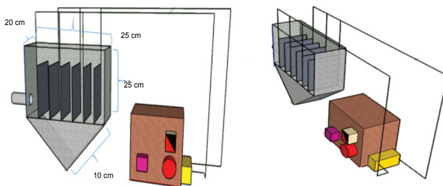
Fig. 1 The making of electrocoagulation reactors front Look (a) and (b) side view.
